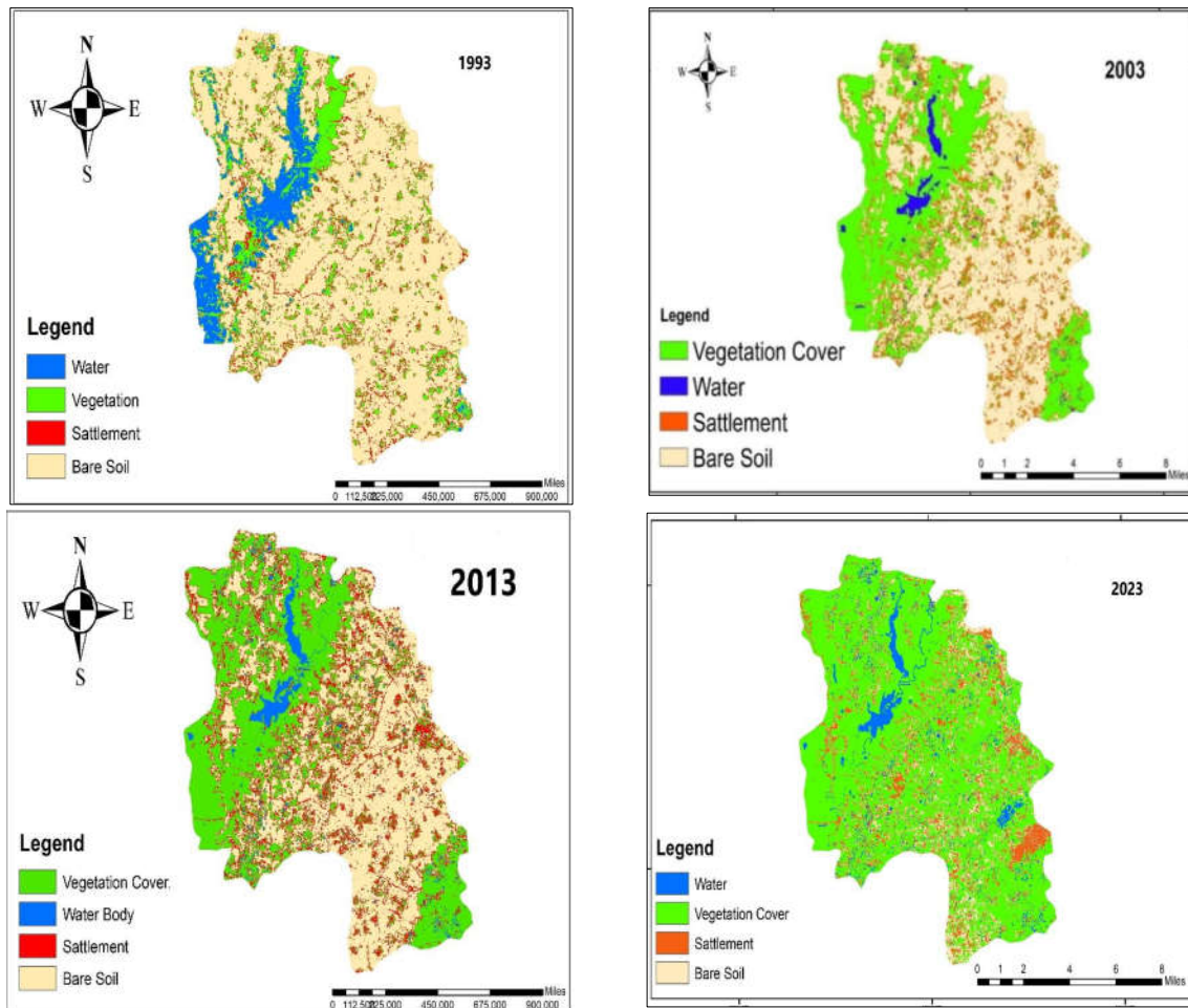
Fig. 4. LULC Maps (1993, 2003, 2013, 2023)
