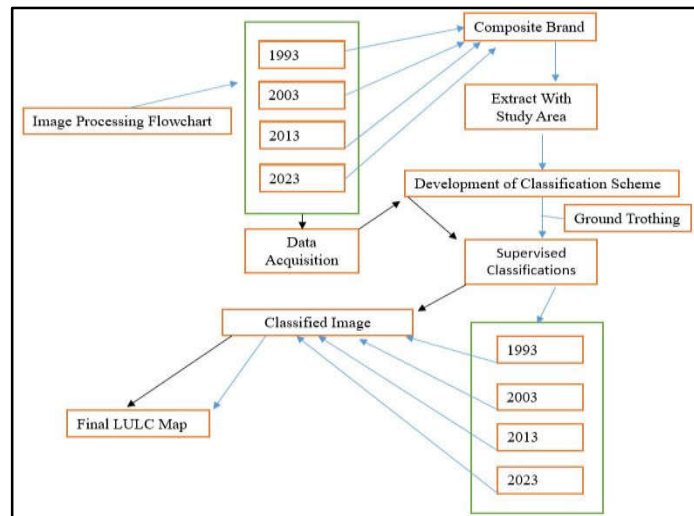
Fig. 3. Satellite image processing
