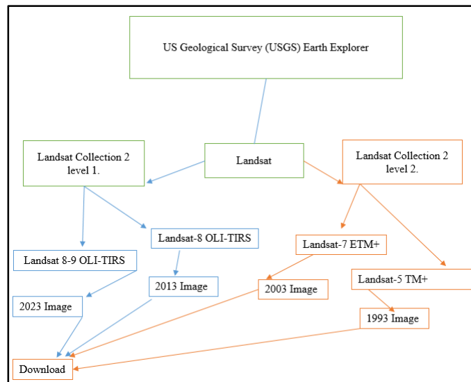
Fig. 2. Satellite Image Sourcing Processing
