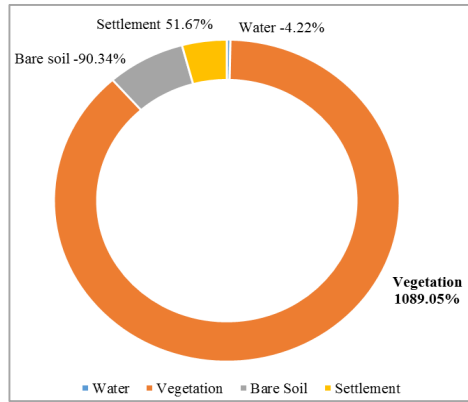
Fig. 6. Annual percentage LULC over four decades (1993÷2023)
